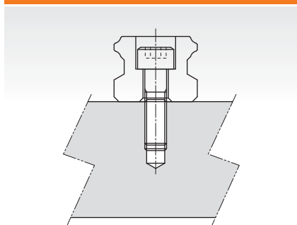
Counter bore (R, U type)
