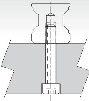
Tapped Hole (T type)
