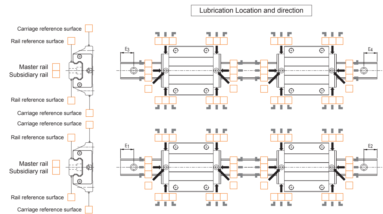
Reference surface & Lubrication Location
