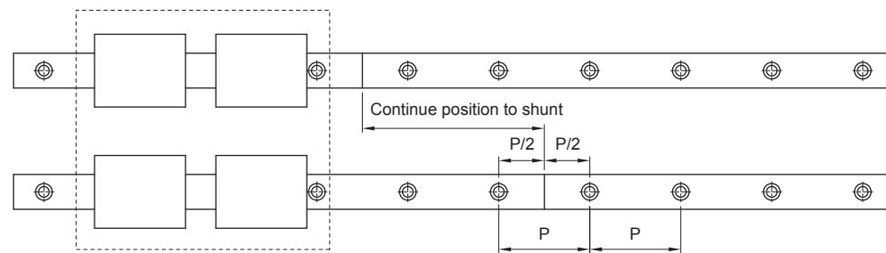
Staggering the joint position
