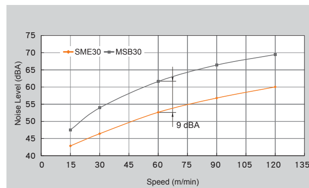
Noise level comparison test
