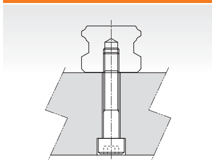
Tapped Hole (T type)
