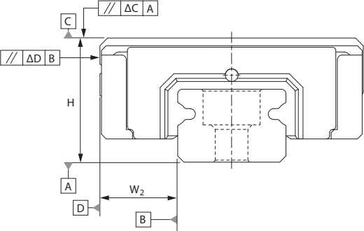
Accuracy of MSC series, divided into 3 classes, normal grade (N), high precision (H), precision (P)
