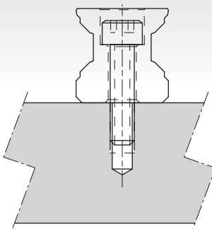
Counter bore (R type)
